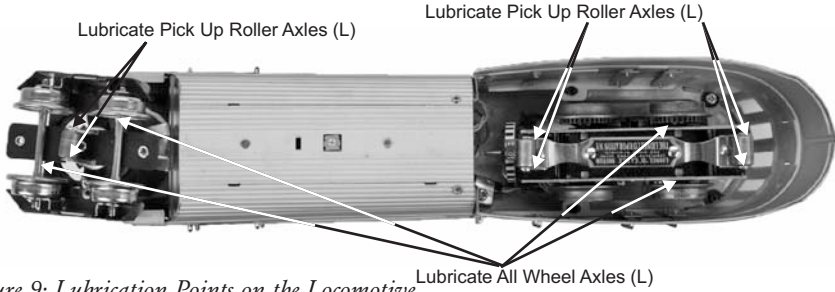
Figure 9: Lubrication Points on the Locomotive
