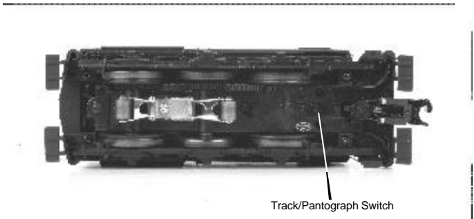
Figure 2. Use pantograph/track switch to select method of power pick-up
