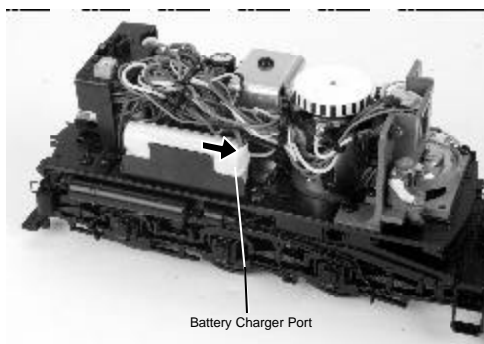
Figure 8: Removing The Battery
