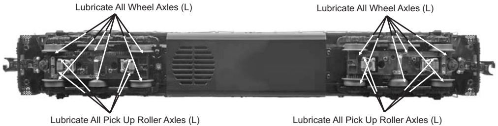
Figure 8: Lubrication Points on the Locomotive
