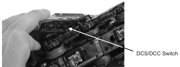
Figure 6: Changing from DCS to DCC Mode
