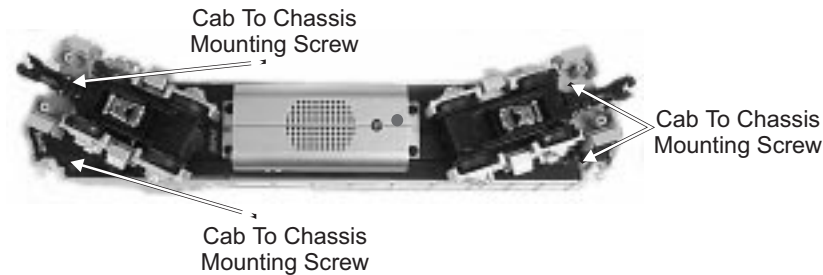
Figure 8: Removing The Body From The Chassis
