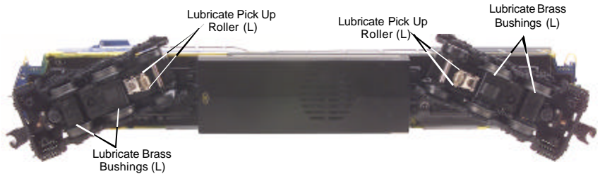
Figure 5. Lubrication Points on the Locomotive
