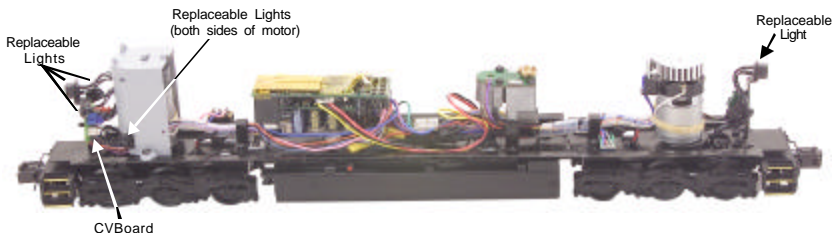
Figure 9. Replacing the Lights in your Engine
