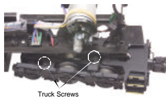
Figure 8. Truckside Mounting Screws to Access the Traction Tires
