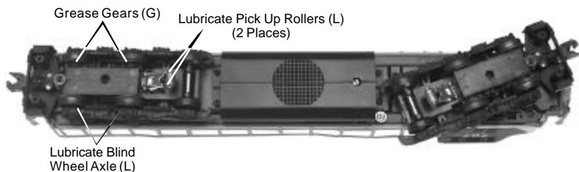
Figure 6: Lubricating The Locomotive Chassis
