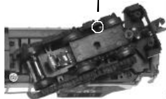
Proto-Coupler® Selection Switch
