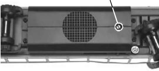
Figure 4: Adjusting The ProtoSound® Volume and selecting the ProtoCoupler direction.
