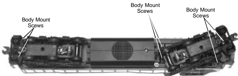
Figure 8: Removing The Body From The Chassis
