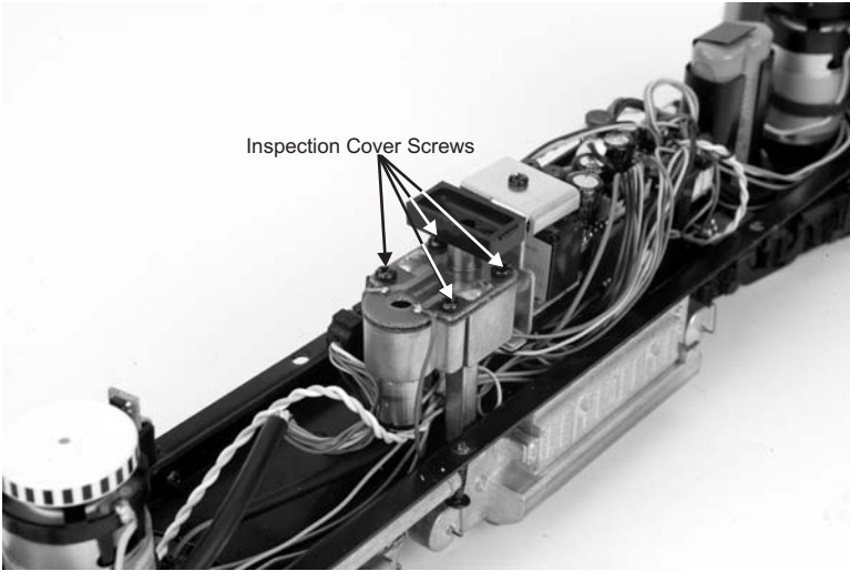
Figure 11. Inspecting the Smoke Unit Wick
