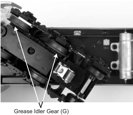
Figure 7. Greasing The Idler Gears
