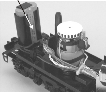
Battery Location
