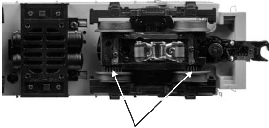
Figure 10: Greasing the Idler Gears Grease Idler Gear (G)
