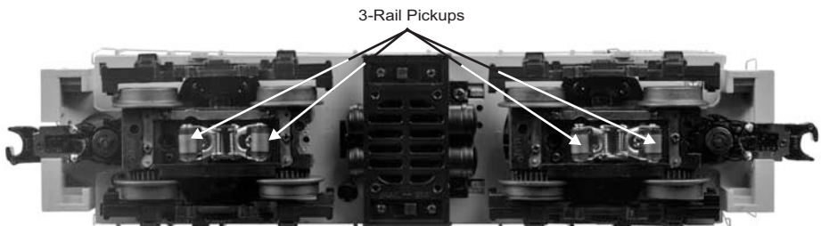
Figure 5: 2-Rail/3-Rail Operation
