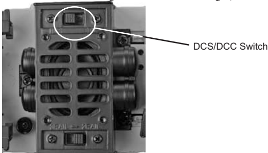
Figure 6: Changing from DCS to DCC Mode
