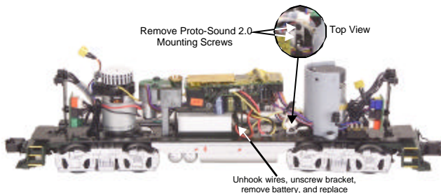
Figure 12. Replacing the Battery (Remove the Proro-Sound 2.0 Board to access the battery.)
