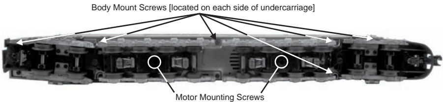
Figure 7: Body Mount and Motor Mounting Screws
