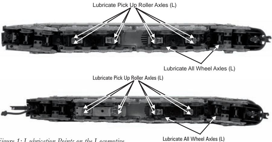
Figure 1: Lubrication Points on the Locomotive
