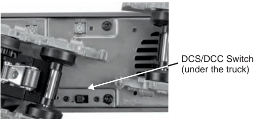
Figure 4: Changing from DCS to DCC Mode
