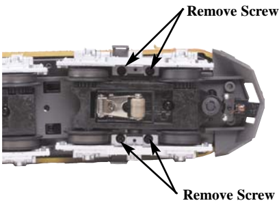
Figure 9 - Traction Tire Replacement
