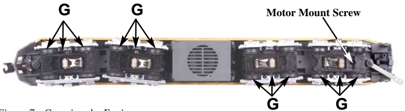
Figure 7 - Greasing the Engine
