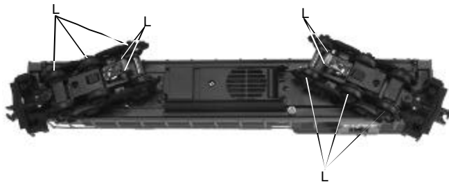
Figure 7: Lubricating The Truck
