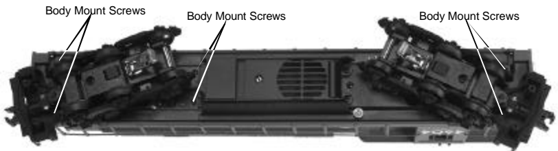
Figure 9: Removing the Body Mount Screws
