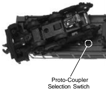
Figure 1: Locating The Proto-Coupler Selection Switch
