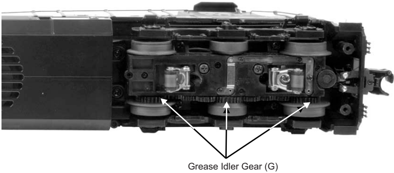
Figure 10: Greasing the Idler Gears
