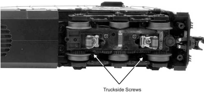
Figure 11: Truckside Screws
