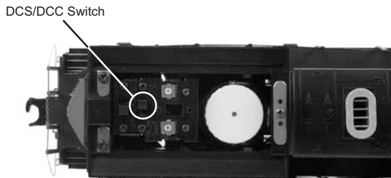
Figure 6: Changing from DCS to DCC Mode
