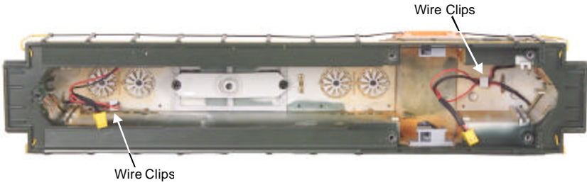
Figure 10. Replacing the Lights Mounted on the inside of the Shell
