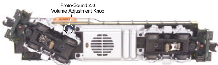
Figure 1. Adjusting the Proto-Sound 2.0 Volume
