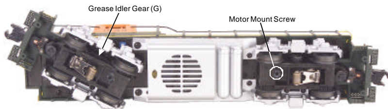
Figure 7. Locations of Greasing Points on the Locomotive
