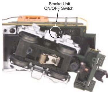
Figure 3. Smoke Unit ON/OFF Switch
