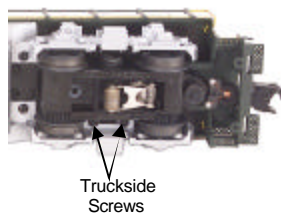
Figure 8. Truckside Mounting Screws to Access the Traction Tires
