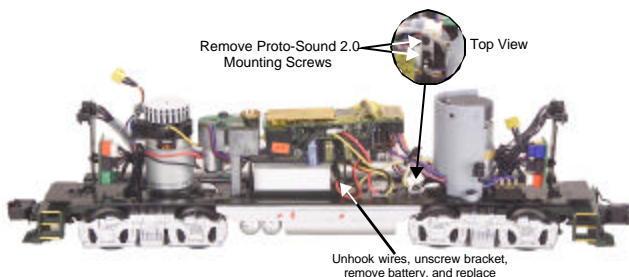
Figure 11. Replacing the Battery (Remove the Proro-Sound 2.0 Board to access the battery.)
