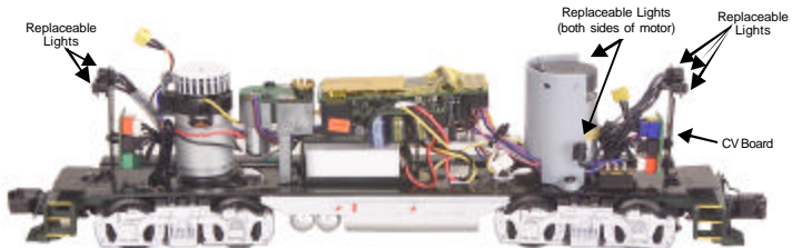
Figure 9. Replacing the Lights in your Engine
