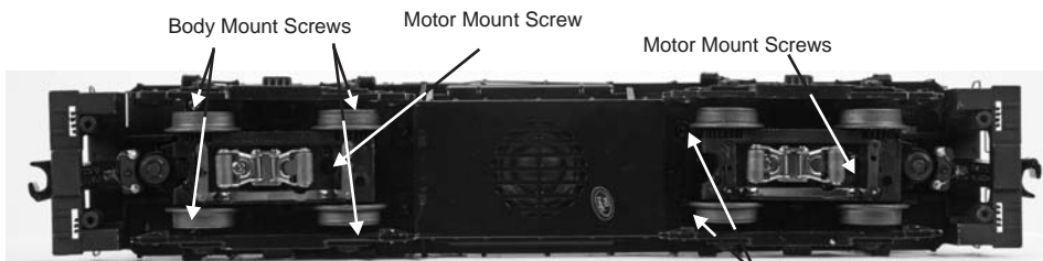
Figure 9: Body Mount Screws
