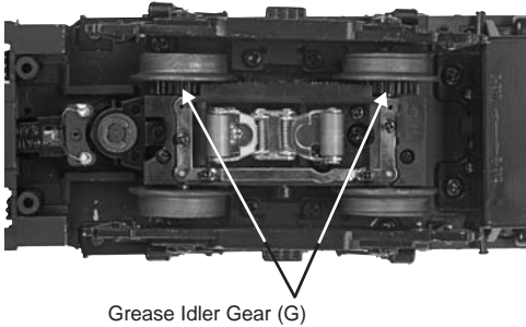
Figure 10: Greasing the Idler Gears
