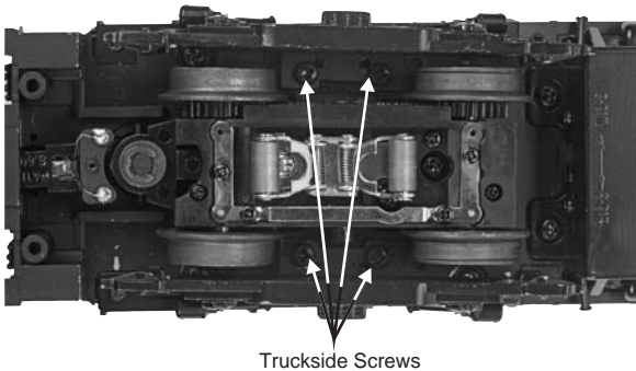
Figure 11: Truckside Screws
