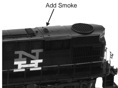
Fig. 12: Adding Fluid
