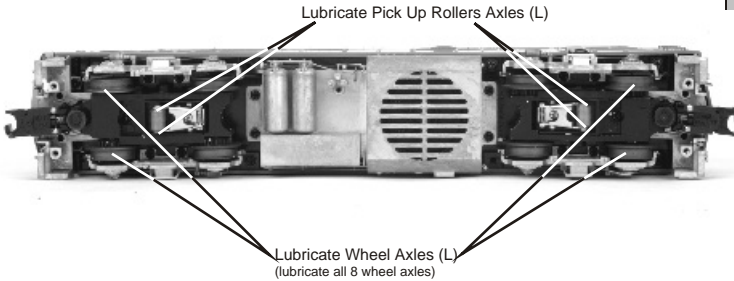
Figure 5. Lubrication Points on the Locomotive.
