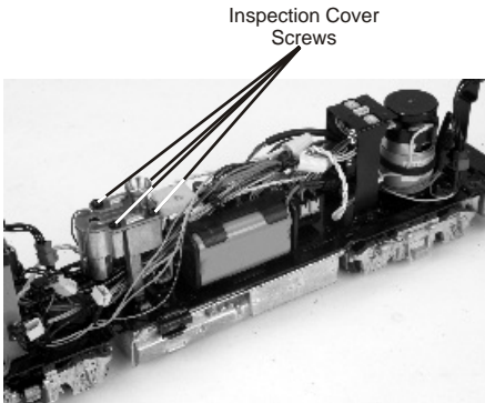
Figure 12. Inspecting the Smoke Unit Wick
