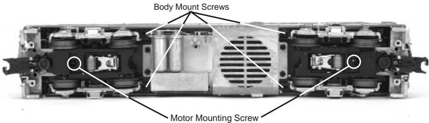
Figure 6. Body Removal Screw Locations
