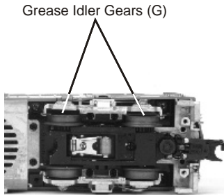
Figure 7. Greasing The Idler Gears
