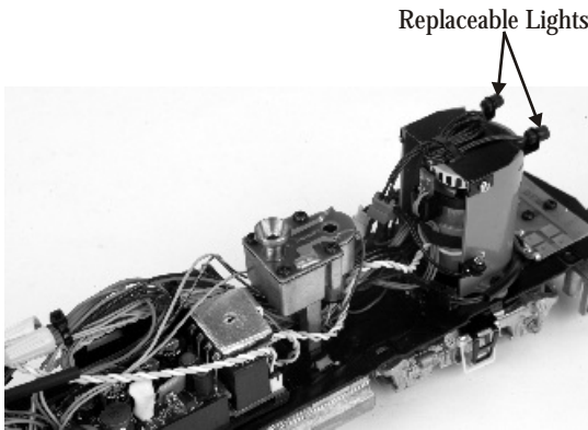
Figure 8: Removing the Replaceable Lights
