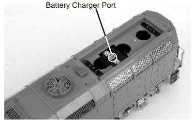
Figure 9. Battery Charger Port location.
