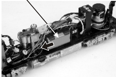
Figure 10. Battery Location.
