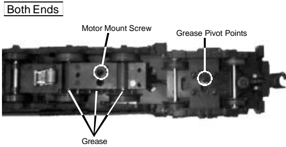
Figure 8: Greasing The Power Trucks
