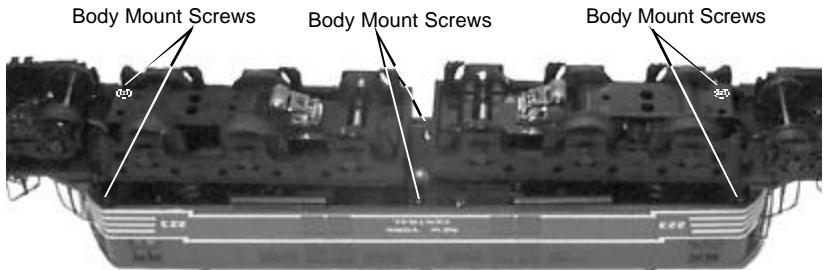
Figure 9: Removing the Body Mount Screws
