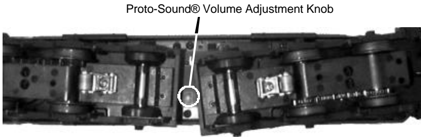
Figure 4: Adjusting The Proto-Sound® Volume
