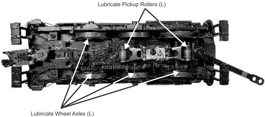
Figure: Lubrication Points on the Locomotive
