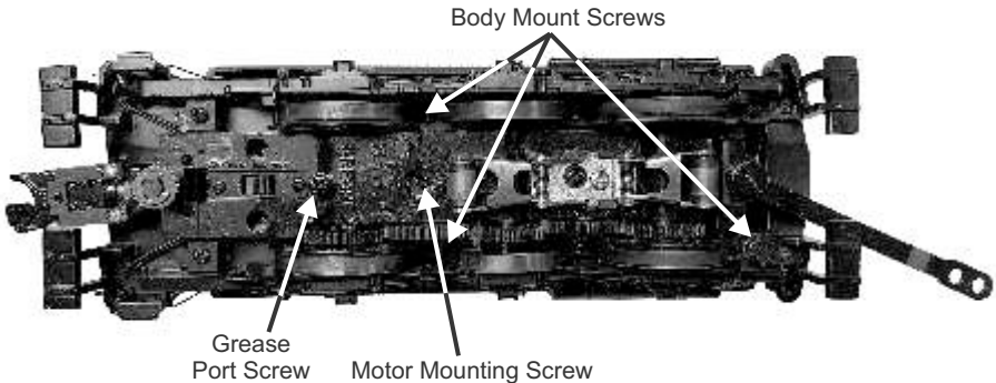
Figure: Body Removal Screw Locations and Motor Mounting Screws
