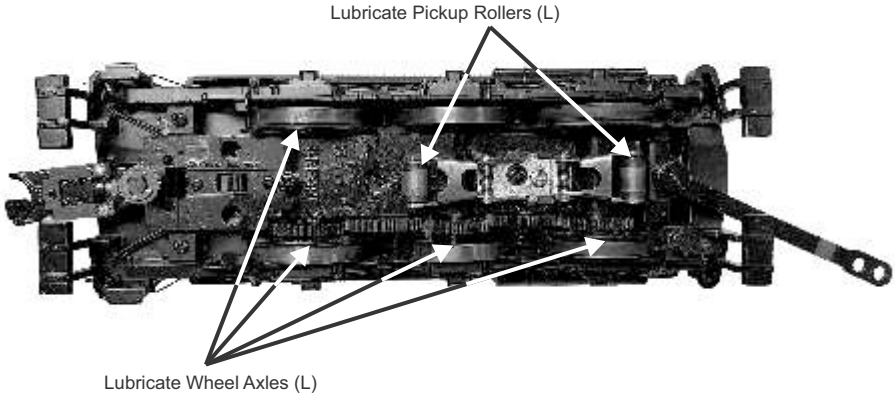
Figure: Lubrication Points on the Locomotive
