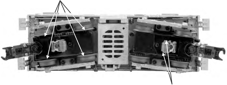
Lubricate All Pick Up Roller Axles (L)
