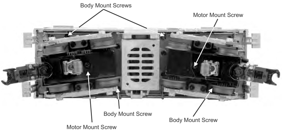
Figure: Body Mount Screws and Grease Points
