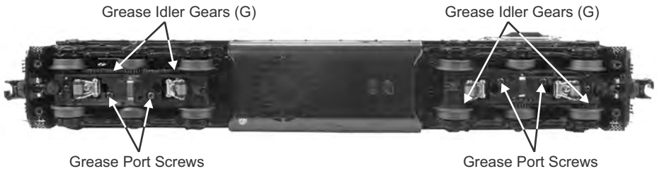
Figure: Greasing The Idler Gears and Port Screws
