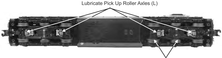
Figure: Lubrication Points
