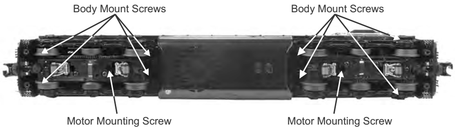
Figure: Body Removal Screw Locations and Motor Mounting Screws
