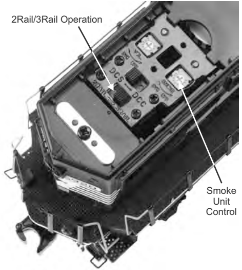
Figure: Smoke Unit Control + 2Rail/3Rail Switch
