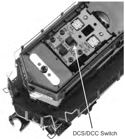
Figure: Changing from DCS to DCC Mode
