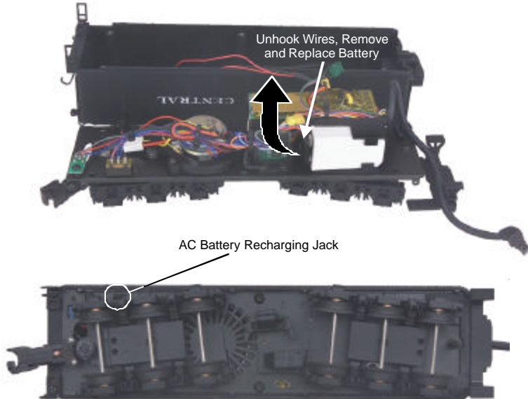
Figure 15: Replacing The Battery And Locating The Battery Recharging Jack
