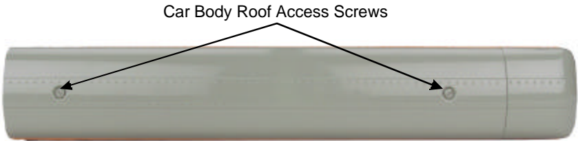
Figure 12: Removing the roof to access the car body interior lights.
