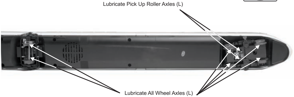
Figure 11: Lubrication Points on the Locomotive
