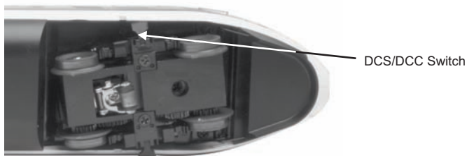
Figure 9: Changing from DCS to DCC Mode
