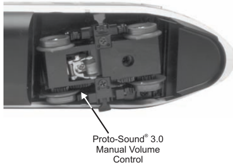
Figure 10: Manual Volume Control
