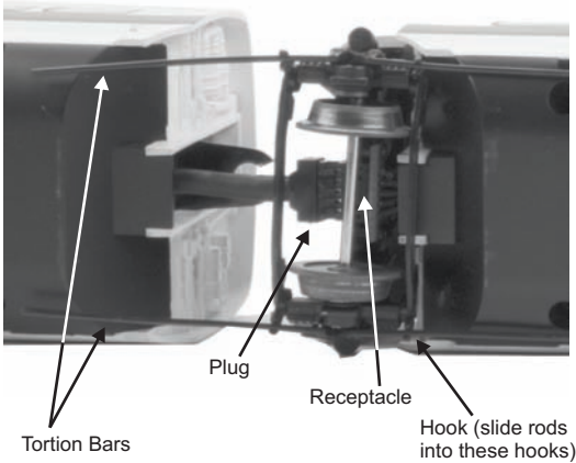
Figure 6: Connecting Plug into Receptacle
