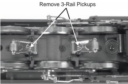
Figure 6: 3-Rail Pickups
