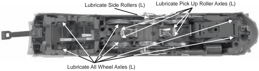
Figure 10: Lubricating the Locomotive
