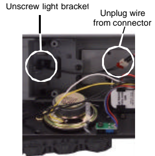
Figure 9. Changing the Tender Light.
