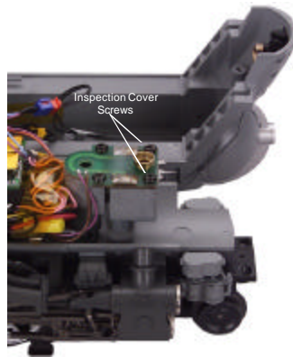
Figure 5. Inspecting the Smoke Unit
