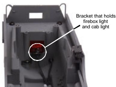
Figure 10. Replacing the Firebox and Cab Lights.
