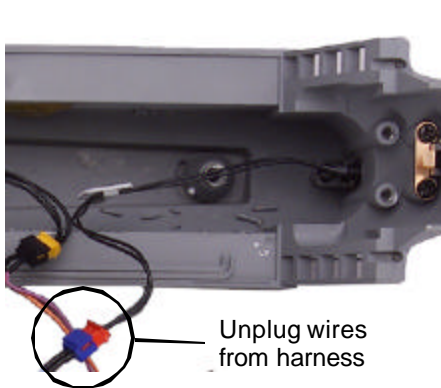
Figure 8. Changing the Headlight.
