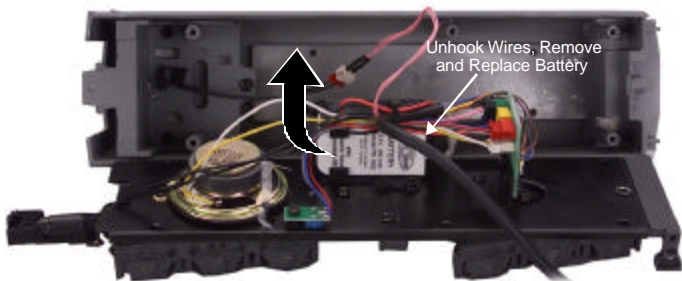
Figure 11. Replacing the Battery
