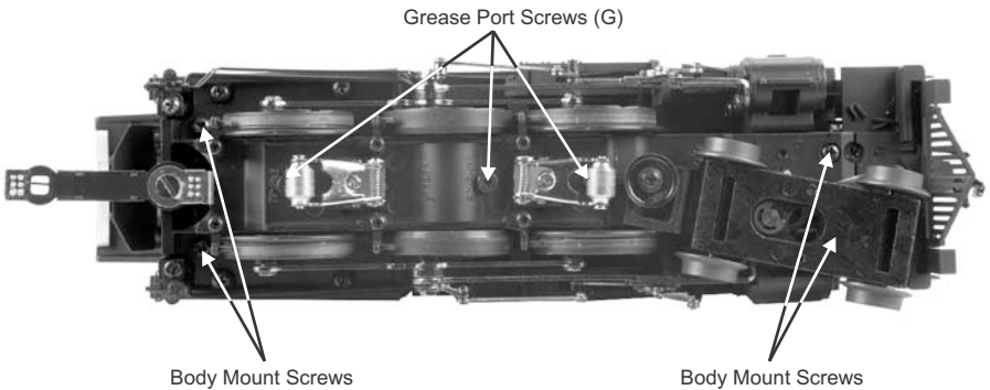
Figure: Grease Points & Body Mount Screw Locations
