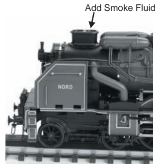
Figure 14: Adding Fluid
