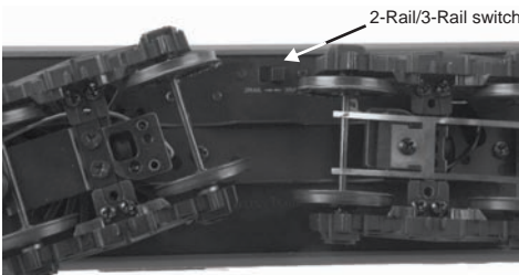
Figure 2: 2-rail / 3-rail switch
