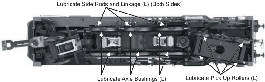
Fig. 11: Lubricating the Locomotive
