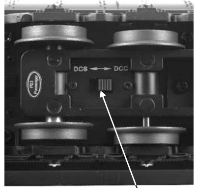
DCS/DCC Switch
