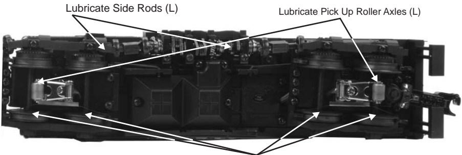
Fig. 9: Lubricating the Locomotive
