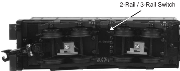
Figure 4: 2-rail / 3-rail switch
