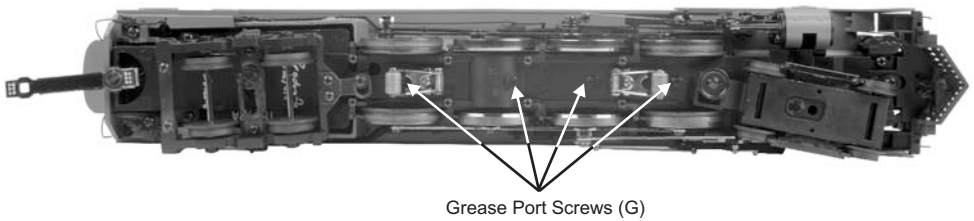
Figure 10: Grease Points
