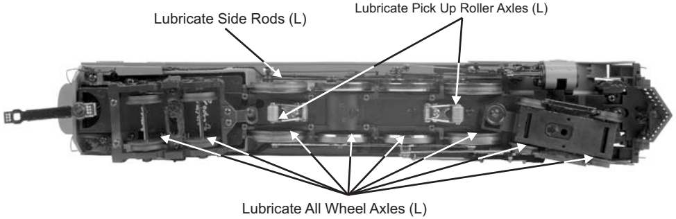
Fig. 9: Lubricating the Locomotive
