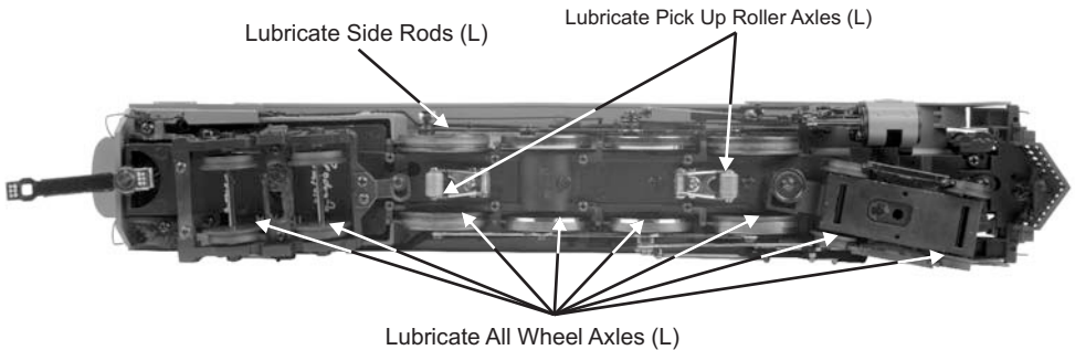
Fig. 1: Lubricating the Locomotive
