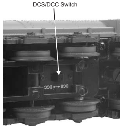
Figure 7: Changing from DCS to DCC Mode
