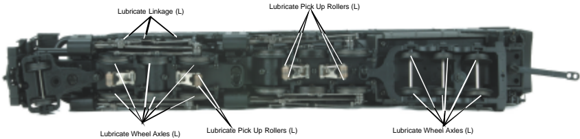
Figure 1. Lubrication Points on the Locomotive
