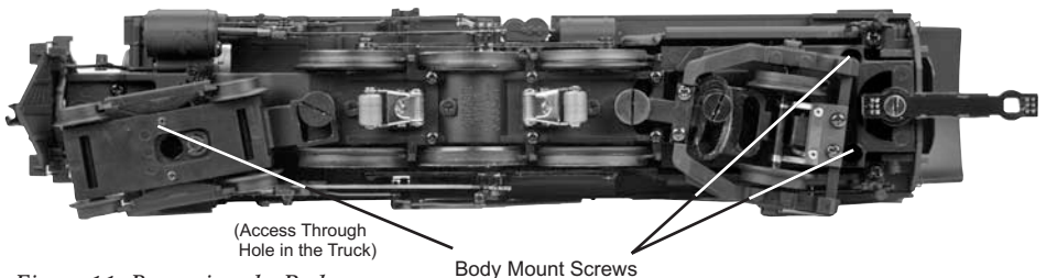
Figure 11: Removing the Body
