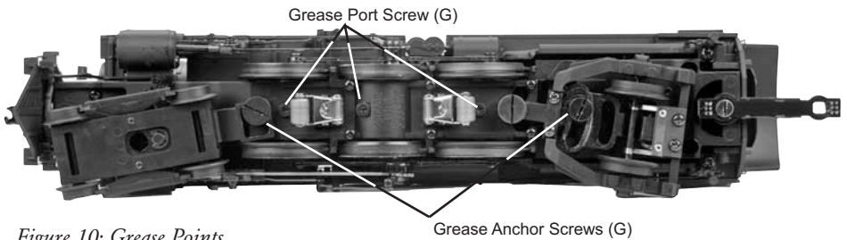
Figure 10: Grease Points
