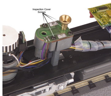
Figure 12: Inspecting The Smoke Unit Wick
