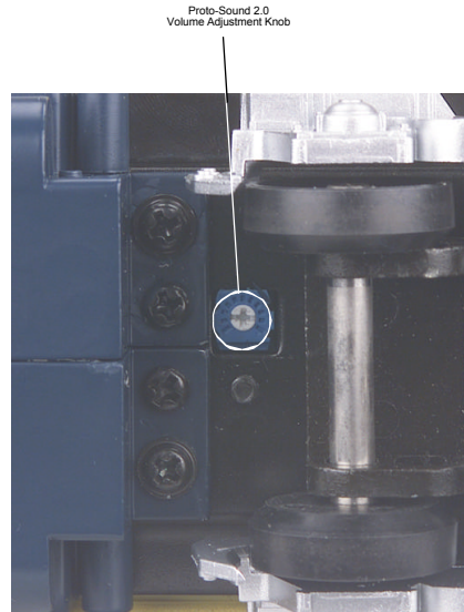
Figure 2: Manual Loco-Sound Volume Adjustment
