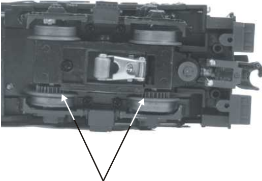
Grease Idler Gear (G)
