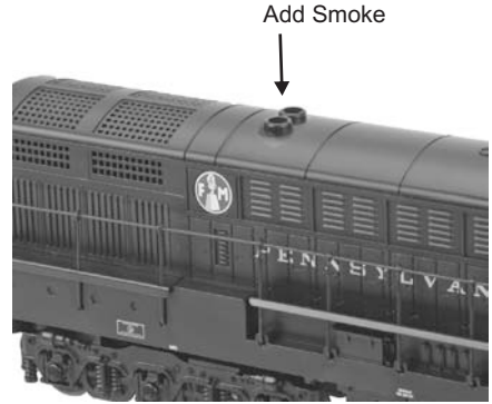
Fig. 10: Adding Fluid
