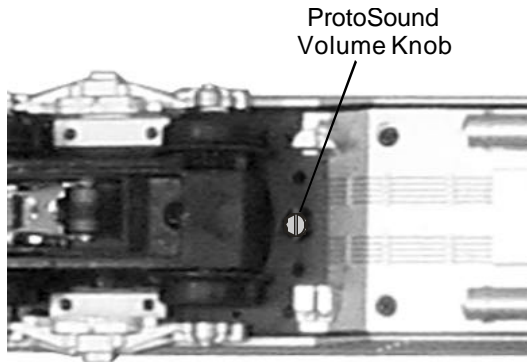
Figure 4: Adjusting The ProtoSound Volume
