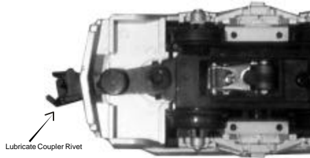
Figure 3: Lubricating The ProtoCouplers
