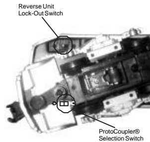
Figure 1: Lock-Out Switch Location
