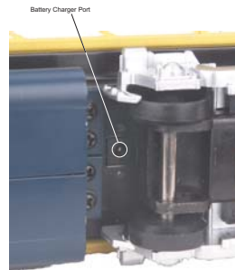
Figure 6: Battery Charger Port
