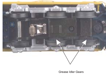
Figure 4: Greasing The Idler Gears
