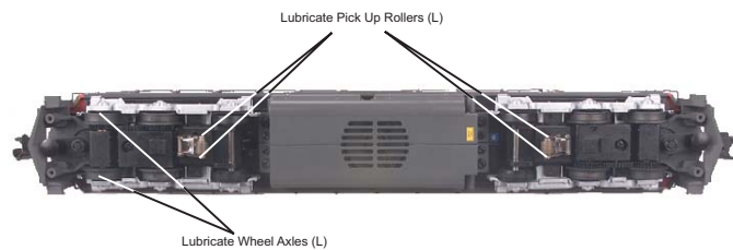
Figure 1. Lubrication Points on the Locomotive
