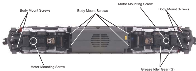
Figure 3: Body Removal Screw Locations
