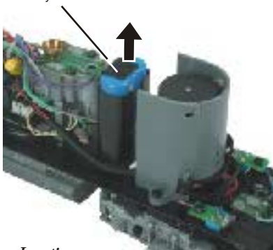
Figure 10. Battery Location.
