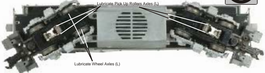
Figure 5. Lubrication Points on the Locomotive.
