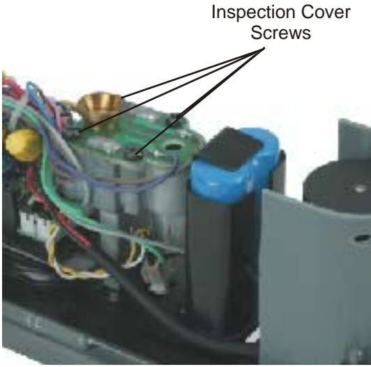
Figure 11. Inspecting the Smoke Unit Wick
