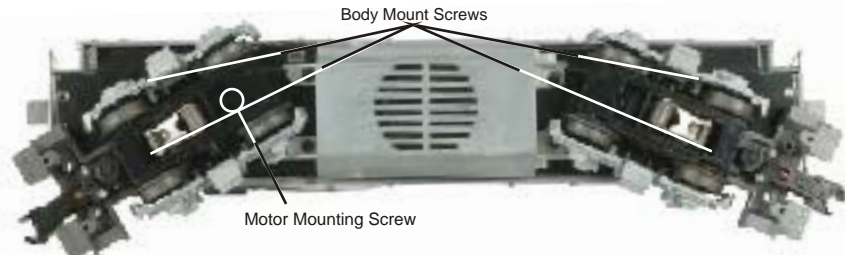
Figure 6. Body Removal Screw Locations
