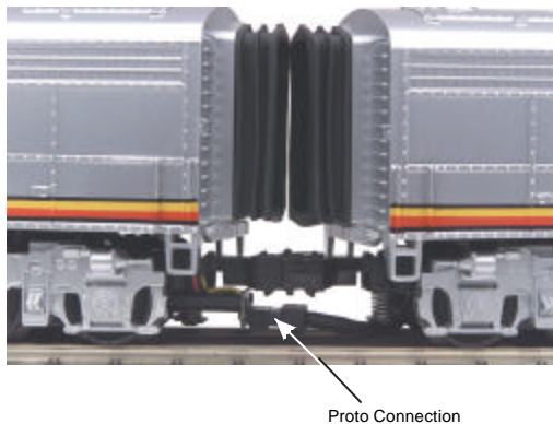
Figure 3: Connecting the Proto-Sound Harness
