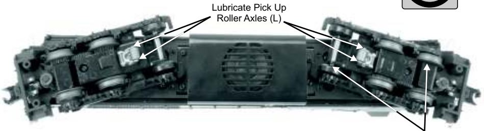
Figure 7: Lubrication Points
