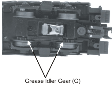
Figure 6. Greasing The Idler Gears
