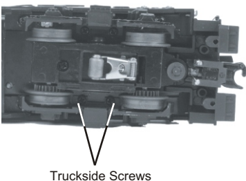
Figure 7. Truckside Screws
