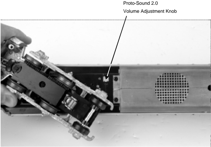
Figure 4: Manual Volume Adjustment Knob
