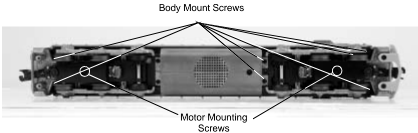
Figure 5: Body Removal Screw Locations
