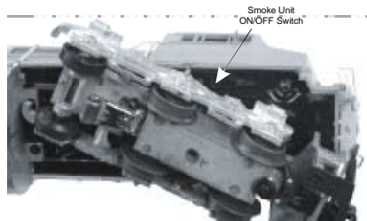
Figure 3: Smoke Unit Switch Location
