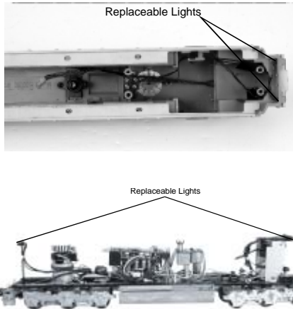
Figure 7: Removing The Replaceable Lights
