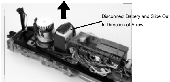
Figure 9: Removing The Battery
