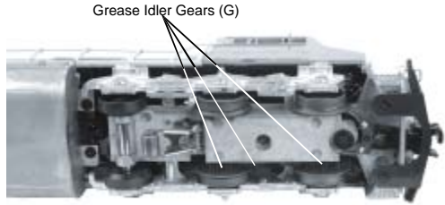
Figure 6: Greasing The Idler Gears
