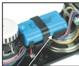
Unhook wires, Remove and Replace Battery
