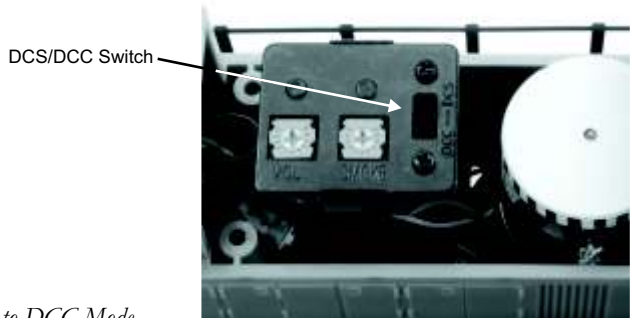
Figure 4: Changing from DCS to DCC Mode
