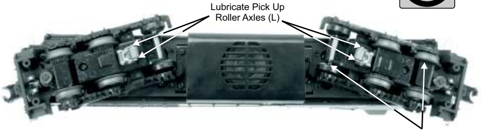
Figure 6: Lubrication Points
