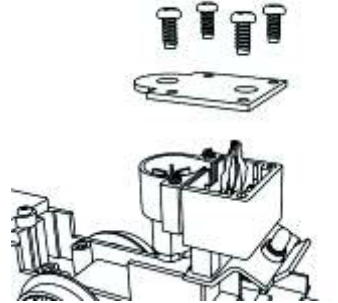
Smoke Unit Cover
