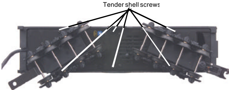
Figure 8: Removing The Tender Body
