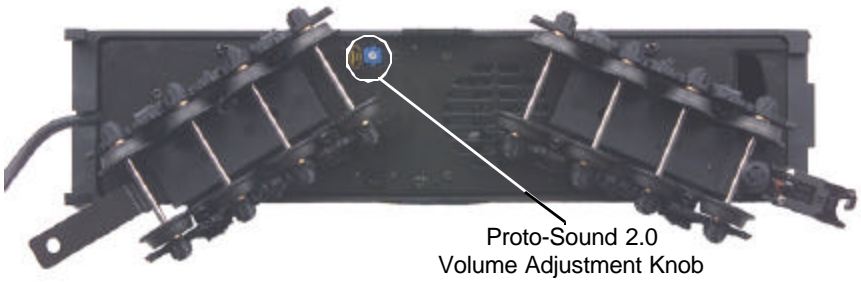
Figure 4: Manual Volume Adjustment
