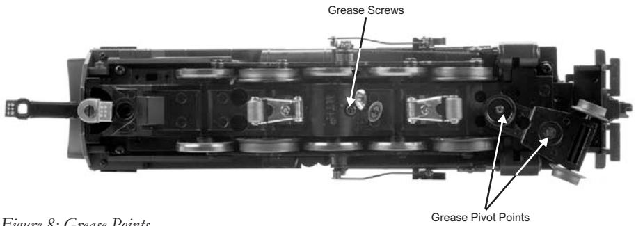
Figure 8: Grease Points
