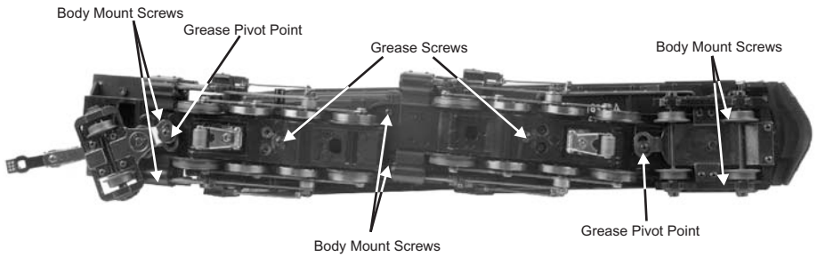
Figure 8: Body Mount Screws and Grease Points
