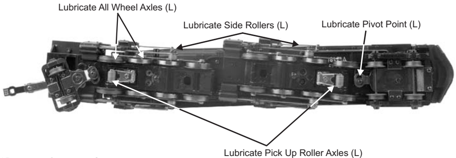
Fig. 1: Lubricating the Locomotive
