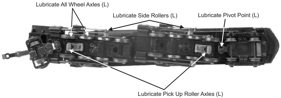
Figure 7: Lubricating the Locomotive
