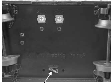
Location for DCS/DCC switch
