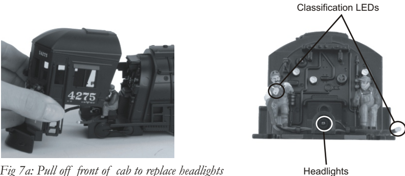
Fig 7a: Pull off front of cab to replace headlights
