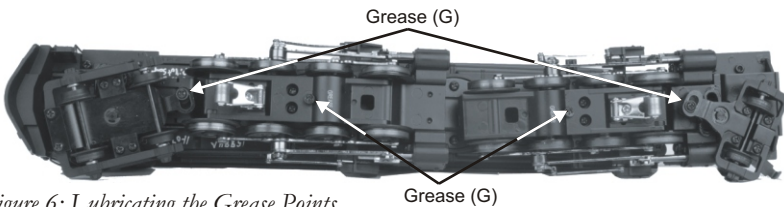
Figure 6: Lubricating the Grease Points and Motor Gearing Grease Plate Screws
