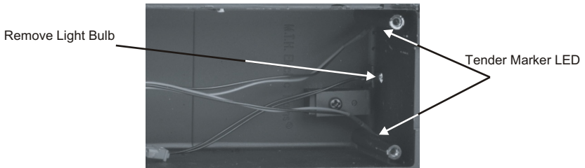
Fig 8a : Location of Tender Marker LED
