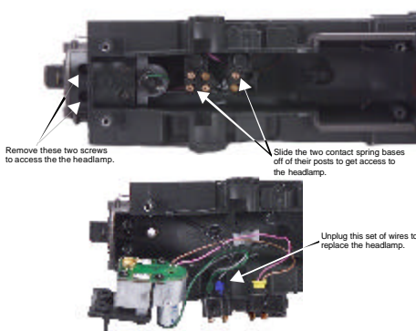
Figure 9. Replacing the Headlight
