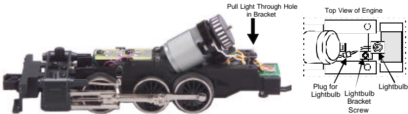
Figure 10. Replacing the Firebox Light in the Rear of the Engine
