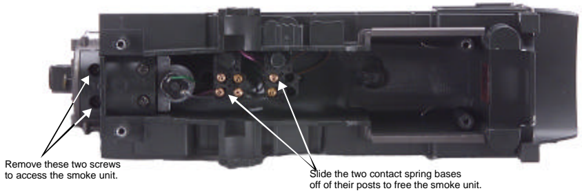
Figure 7. Removing the Smoke Unit Mounting Plate to Access the Smoke Unit
