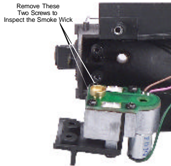
Figure 8. Inspecting the Smoke Unit's Wick
