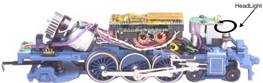
Figure 7. Replacing the Headlight and the Fire Box Light
